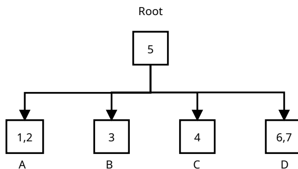
Figure 176: A quad tree
